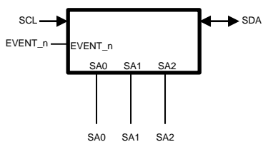
Serial SPD with Thermal sensor
